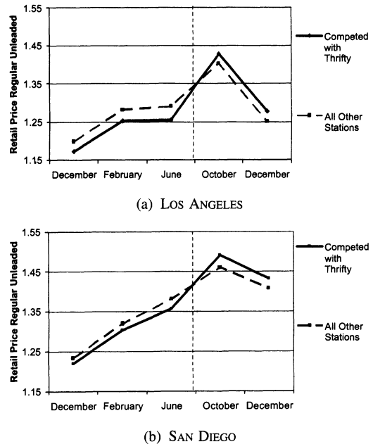
FIGURE 1. TREATMENT AND CONTROL GRAPHS FOR LOS ANGELES AND SAN DIEGO
